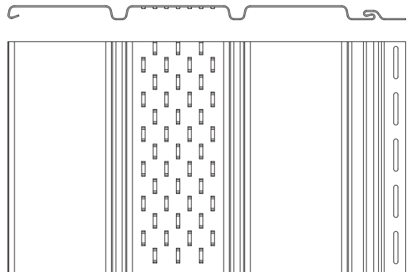
Ventilated panel
