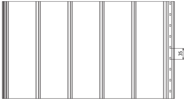
Standard panel
